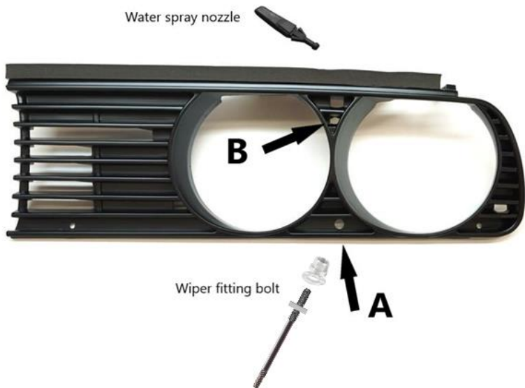
Photo 3 (Water nozzle spray & wiper arm fitting kit location)
