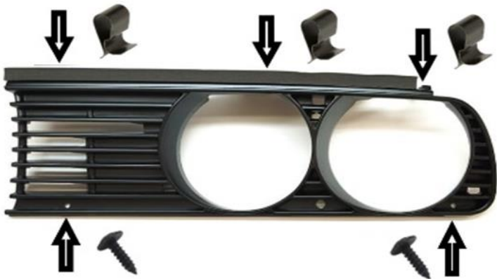
Photo 2 (BMW E30 Headlight grill fitting details)
